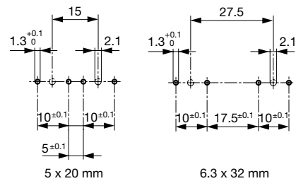
Bohrplan Variante 0751.0056
